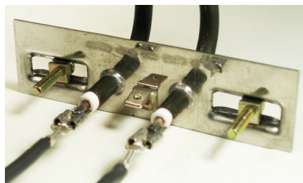
Single Quick Connect
